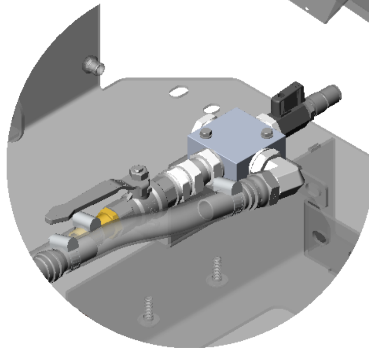
DETAIL I SCALE 1 : 3
